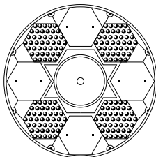
4 modules, 120 LEDs
